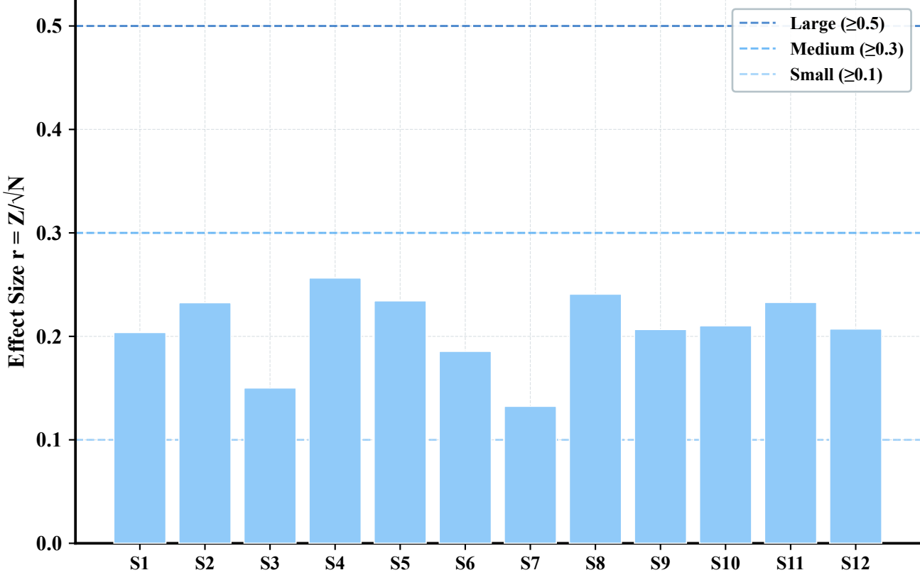
(b) Effect Size (Cohen 1988)
