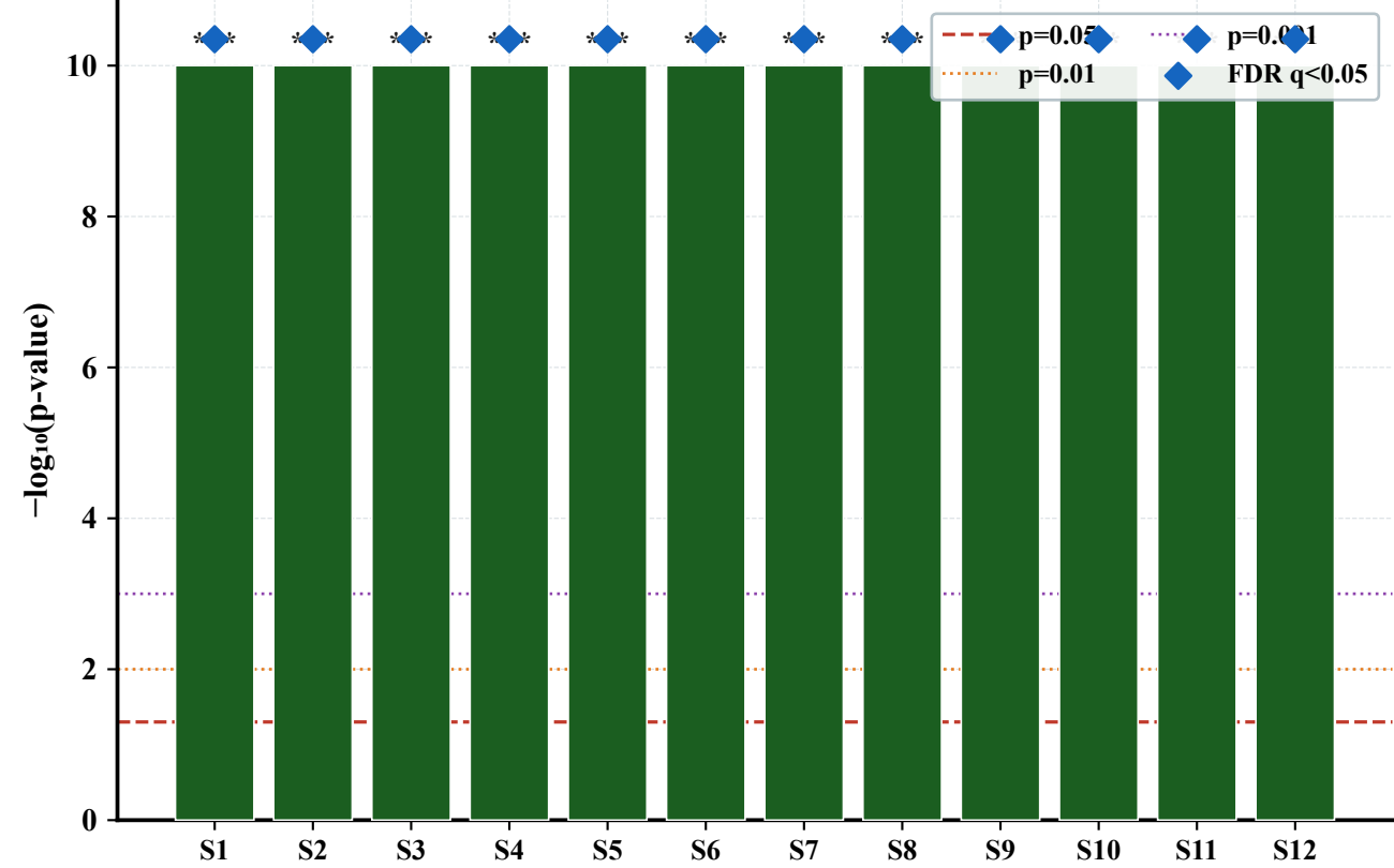
(a) Wilcoxon Signed-Rank Test (one-tailed) H_1: |\text{err\_BC}| < |\text{err\_Raw}|
