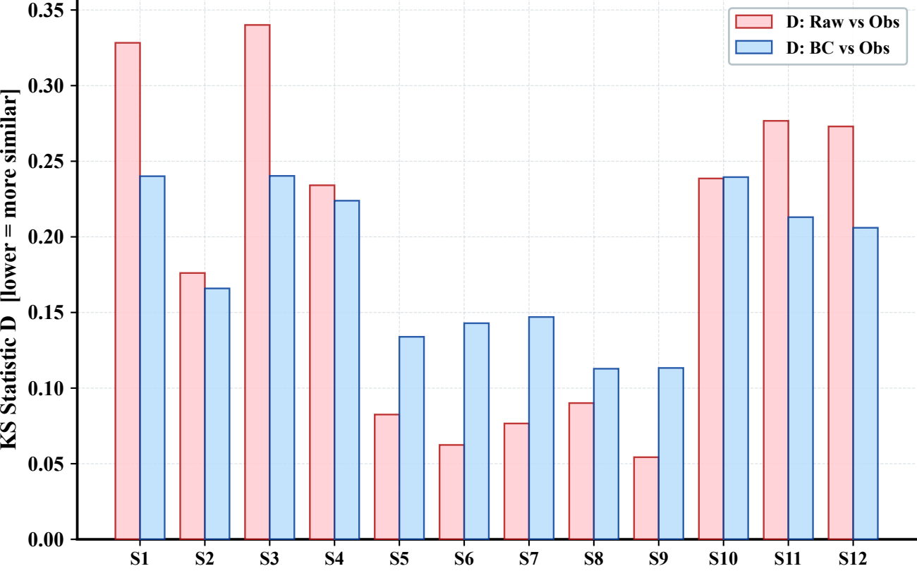
(c) Kolmogorov–Smirnov Test Two-sample: Sim vs Obs (wet days \geq 1 mm/day)
